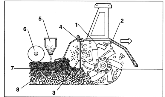
1. Rotor Direction 2. Raised Material 3. Sorting Grid 4. Bonnet 5. Seeder 6. Mesh Roller 7. Sieved Material 8. Deposited Stones
